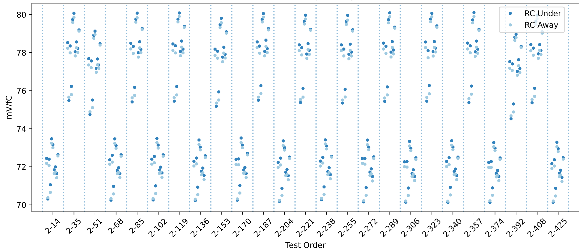
20USBHX2007936 RC gain chip averages
