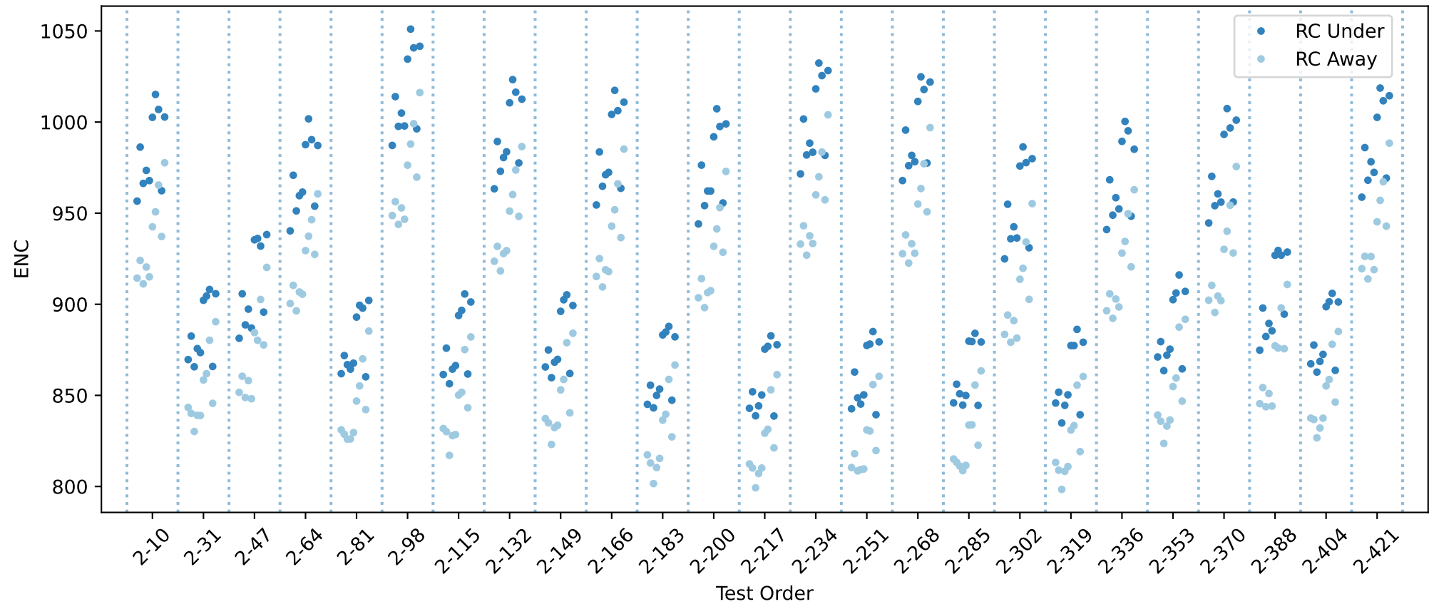
20USBHX2007932 RC innse chip averages
