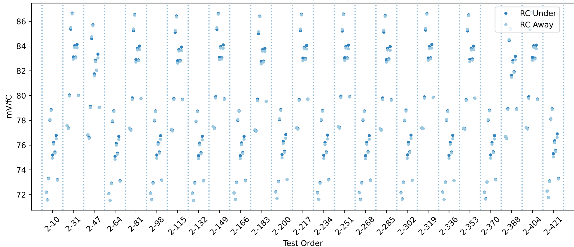
20USBHX2008020 RC gain chip averages
