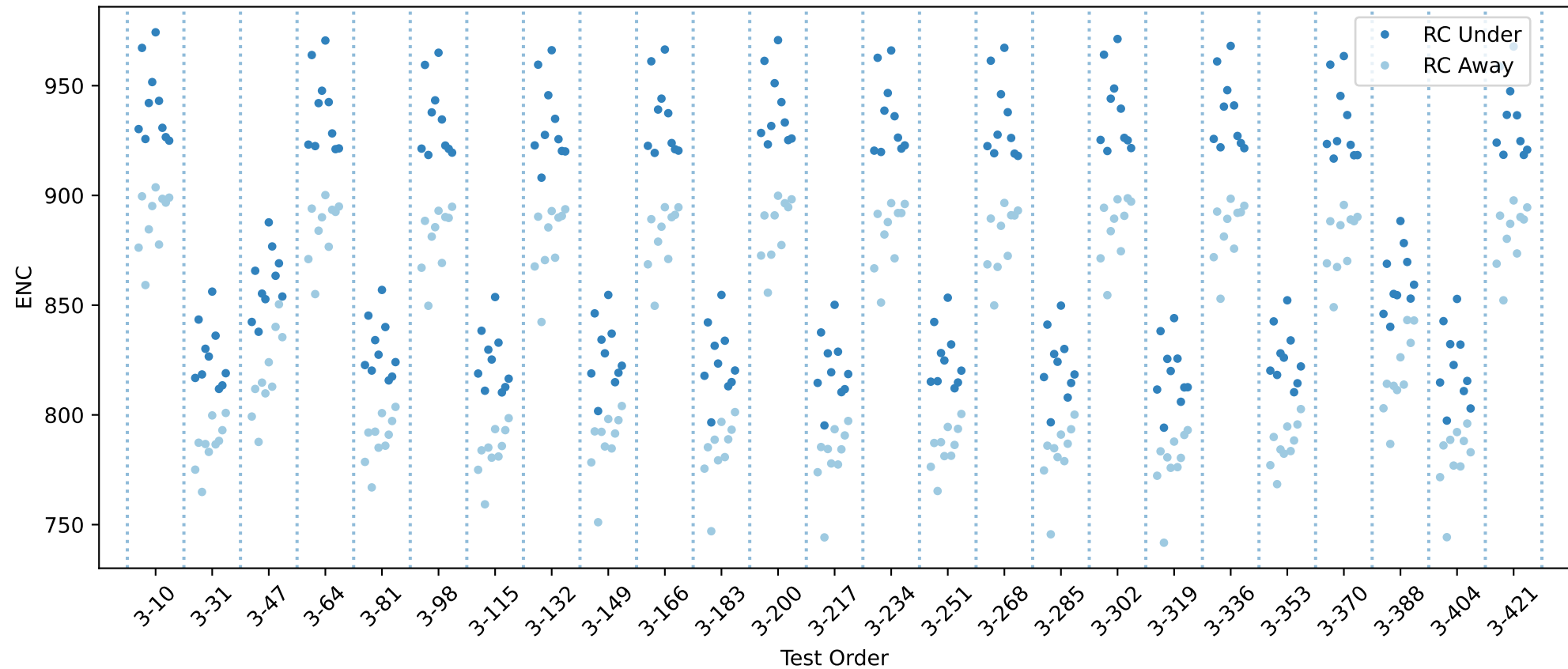
20USBHX2008022 RC innse chip averages
