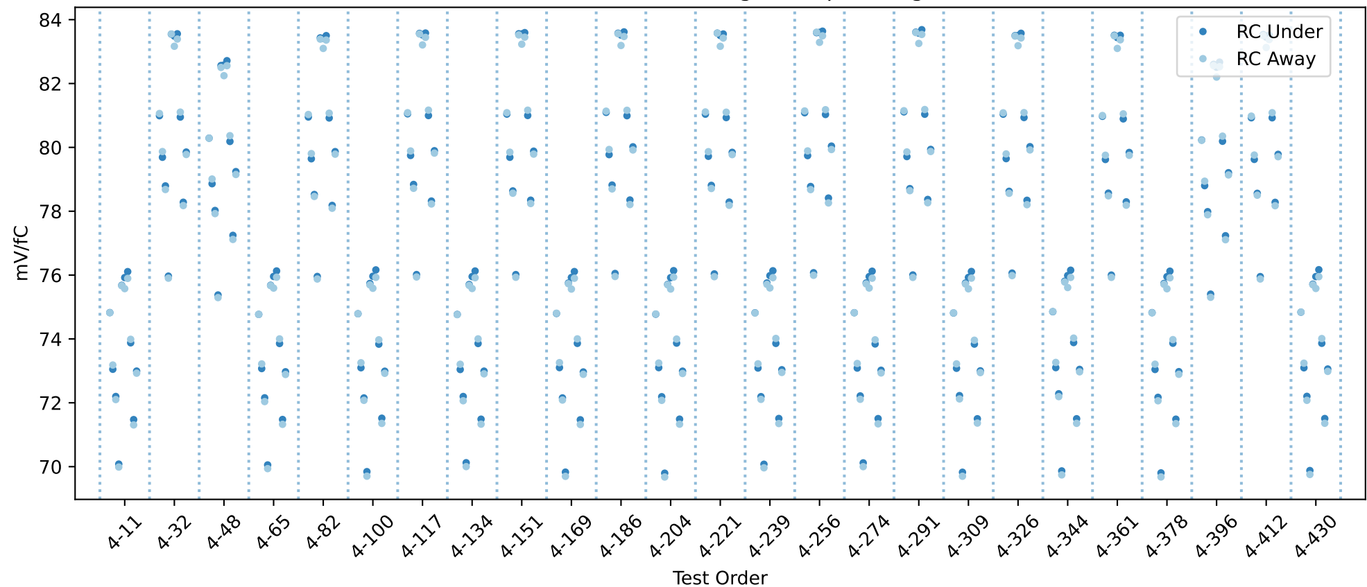
20USBHX2008022 RC gain chip averages
