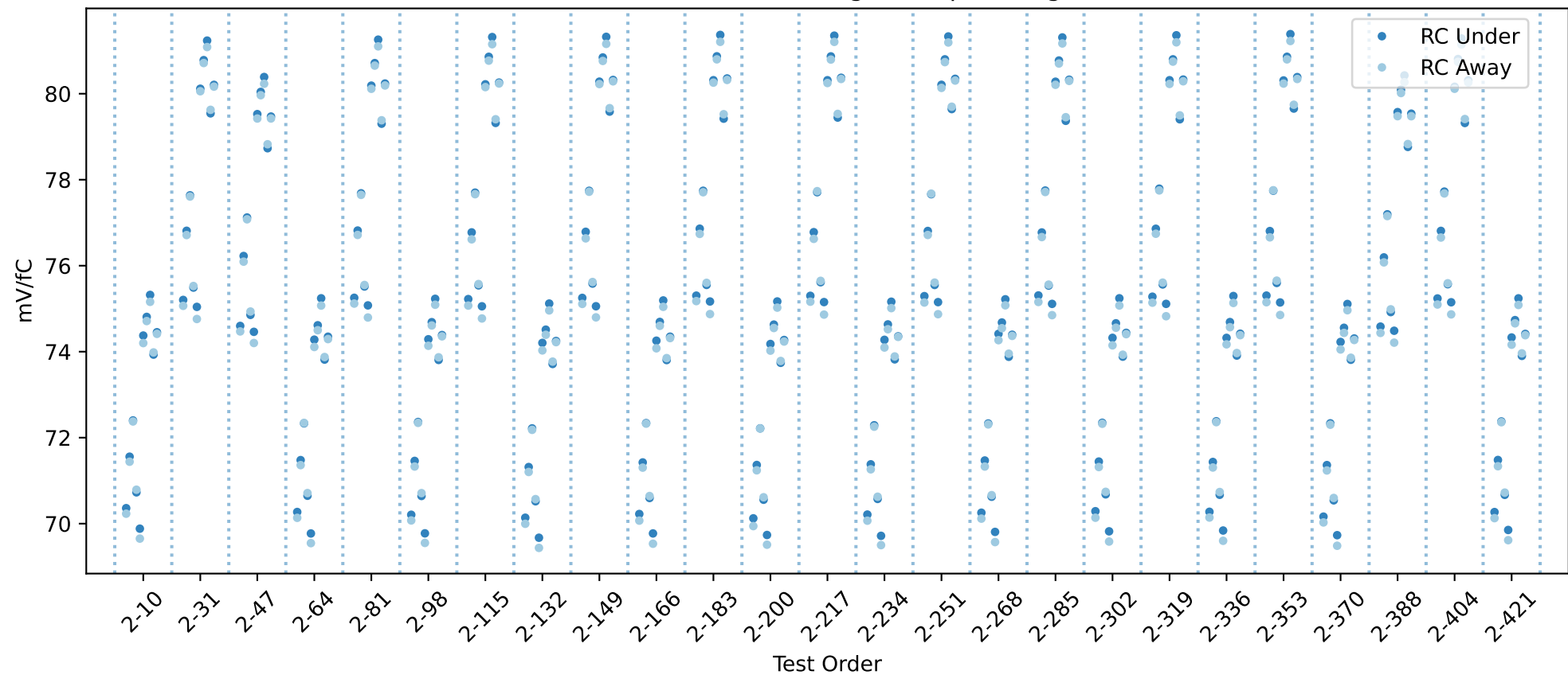
20USBHX2008011 RC gain chip averages
