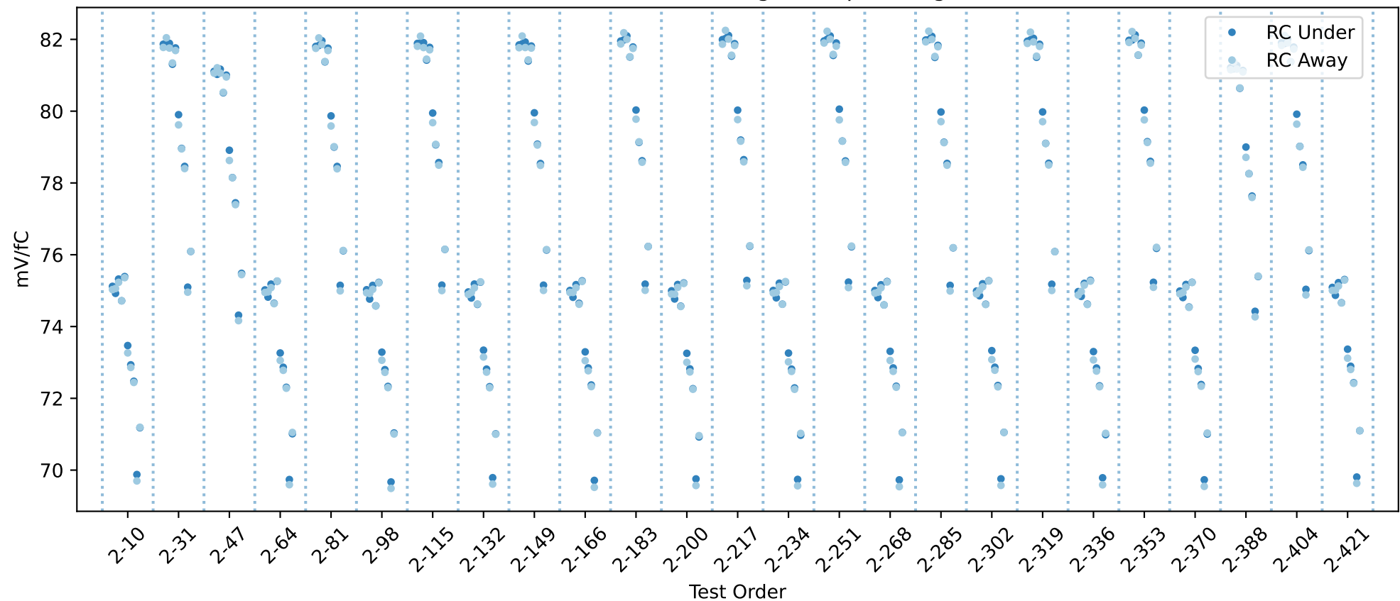
20USBHX2008012 RC gain chip averages
