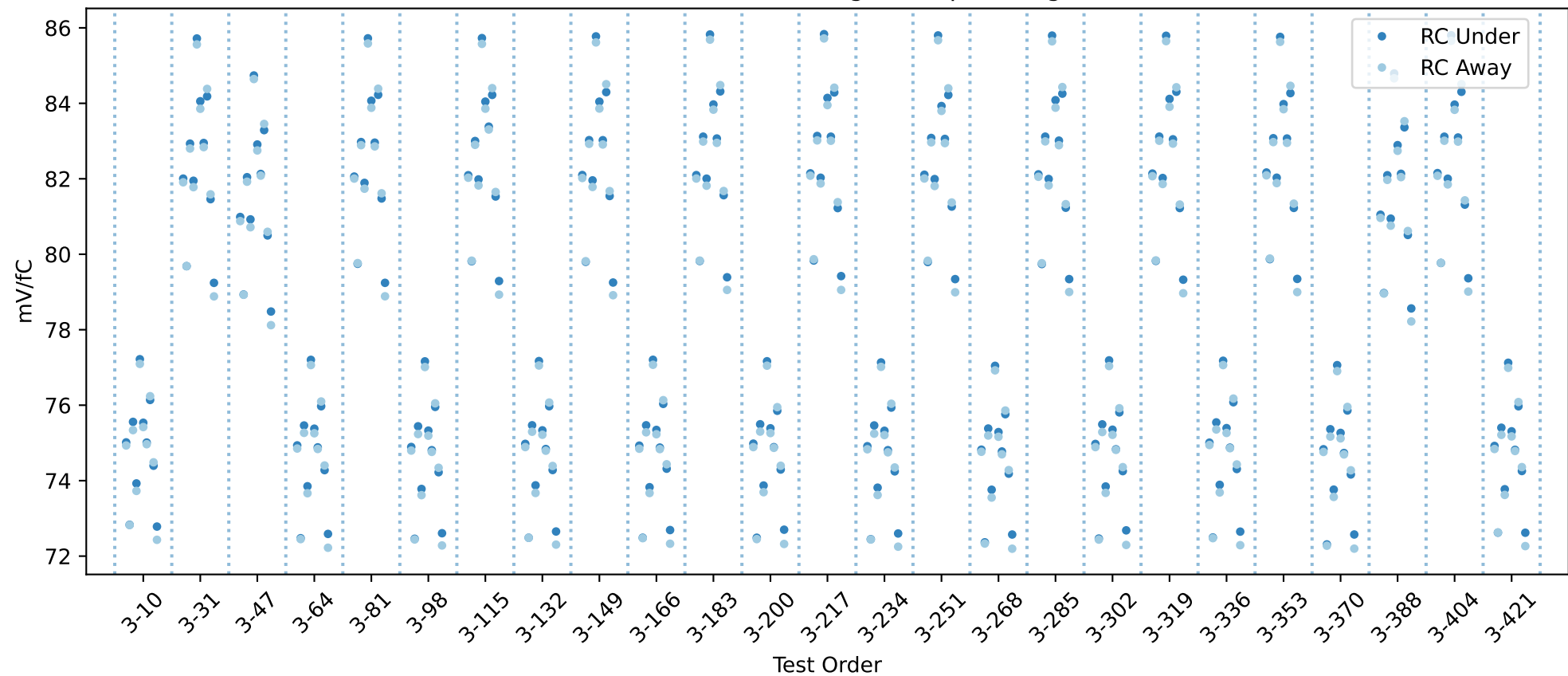
20USBHX2008031 RC gain chip averages
