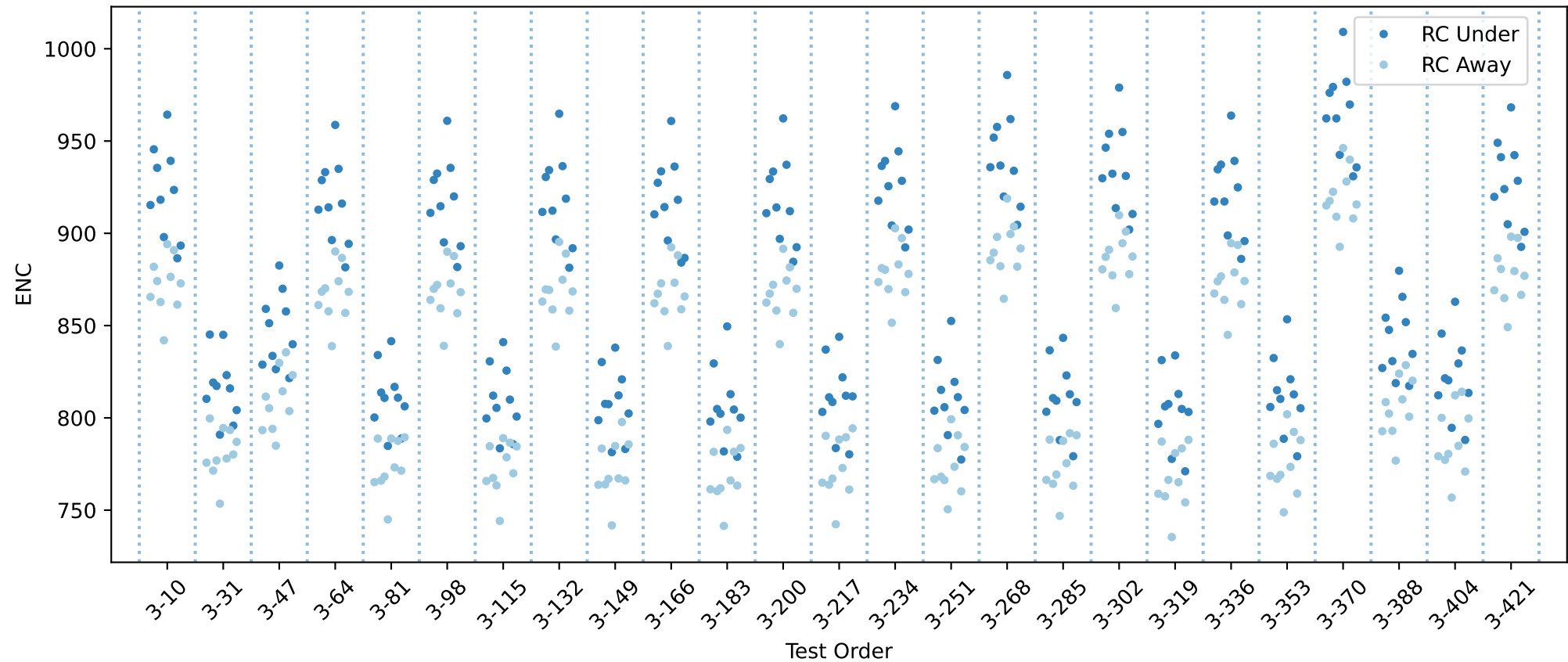
20USBHX2008031 RC innse chip averages
