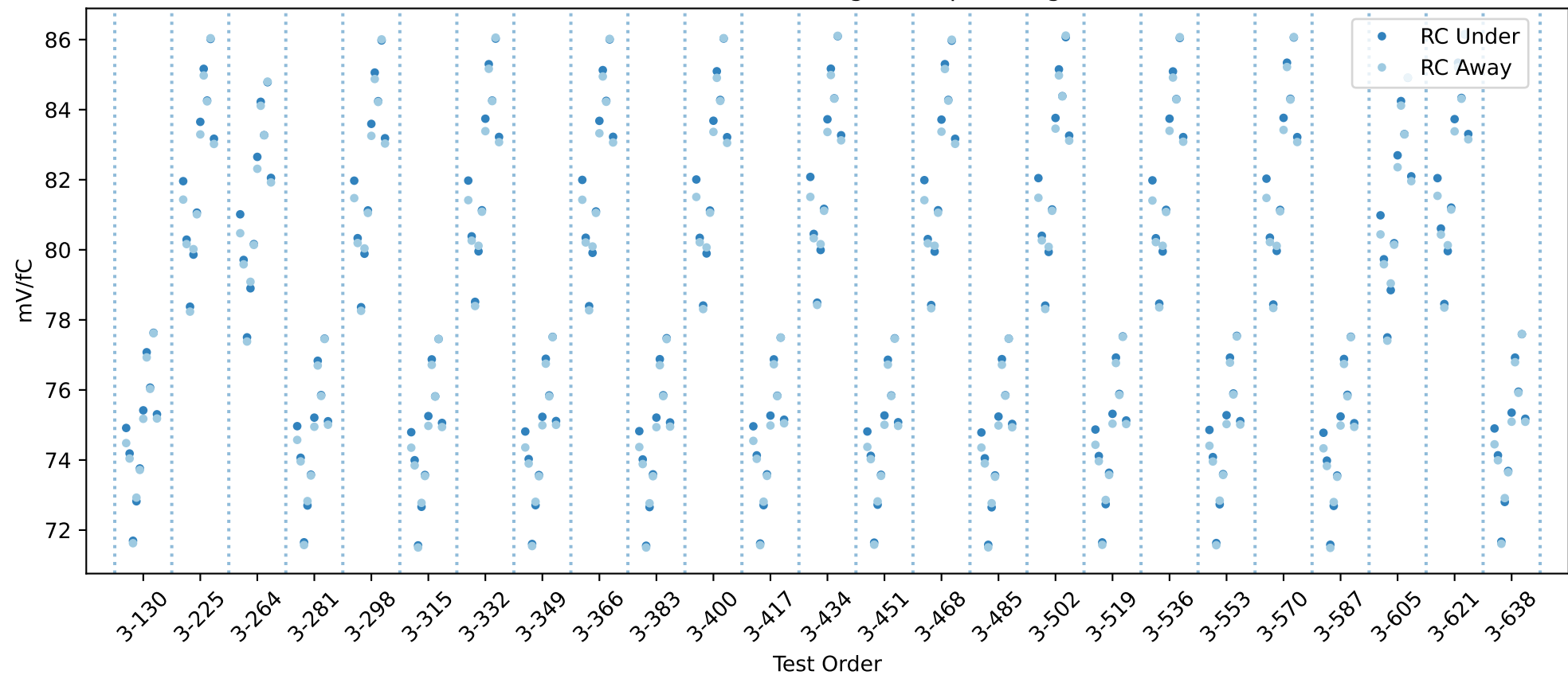
20USBHX2008035 RC gain chip averages
