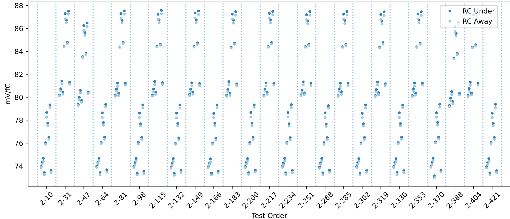
20USBHX2008073 RC gain chip averages
