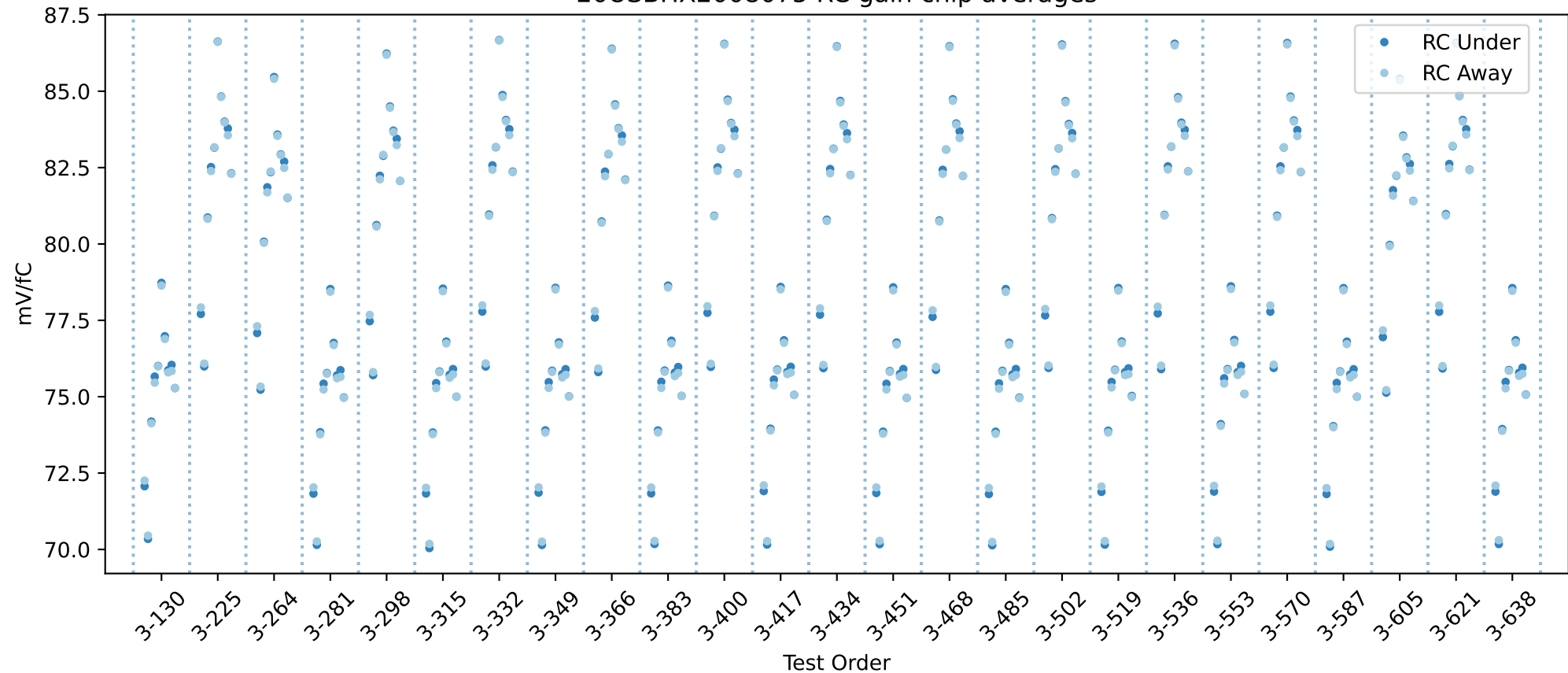
20USBHX2008075 RC gain chip averages
