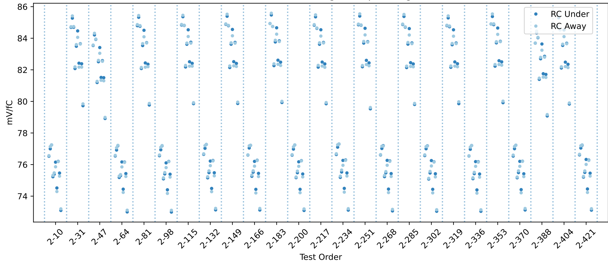
20USBHX2008037 RC gain chip averages
