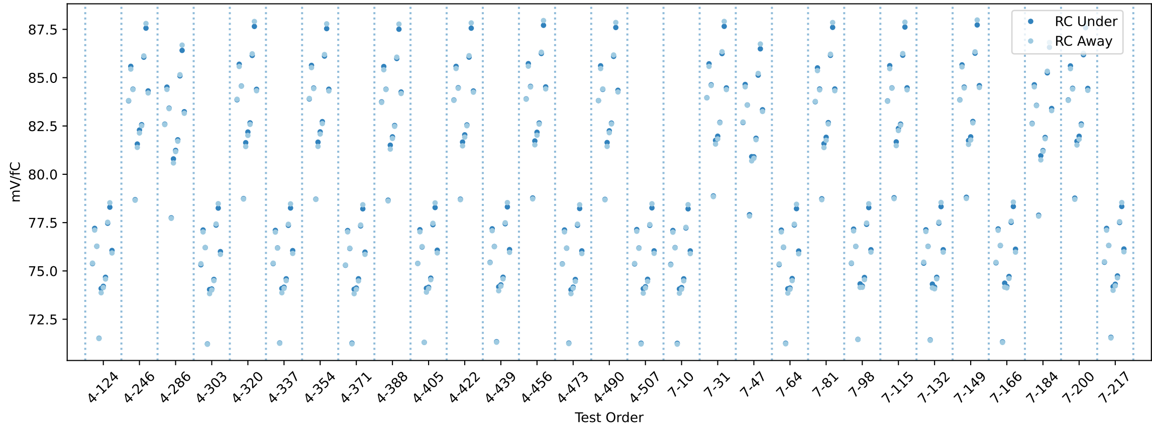
20USBHX2008038 RC gain chip averages
