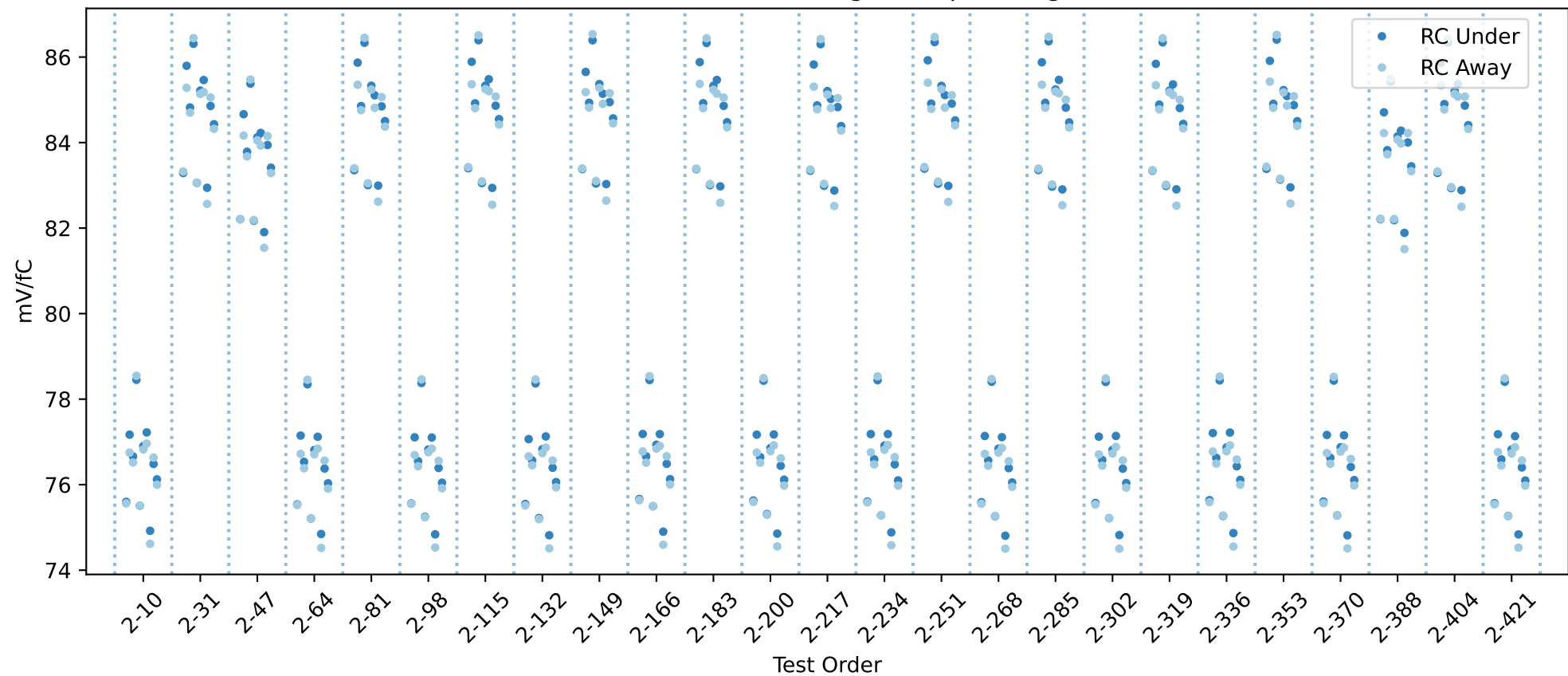
20USBHX2008039 RC gain chip averages
