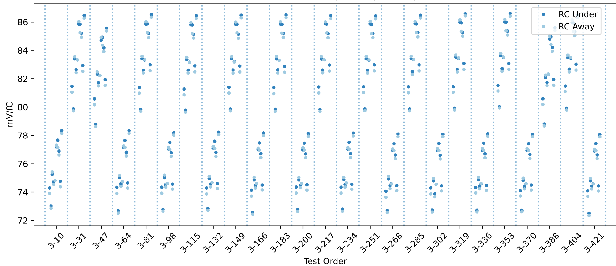
20USBHX2008041 RC gain chip averages
