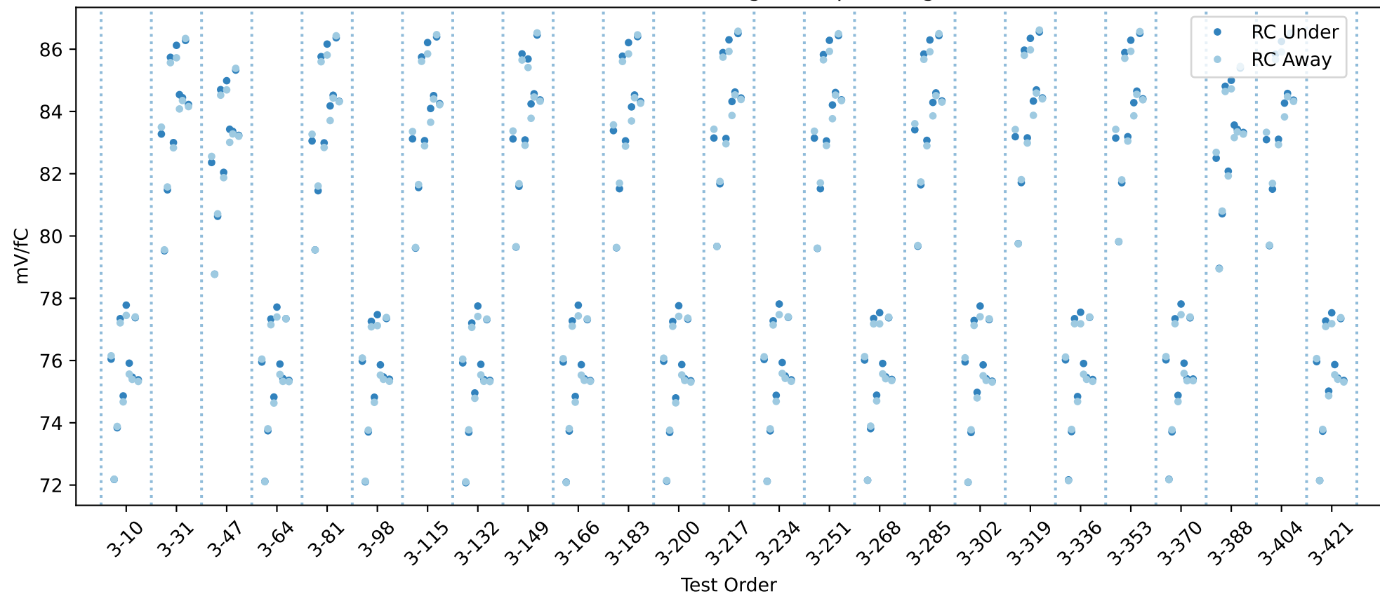
20USBHX2008044 RC gain chip averages
