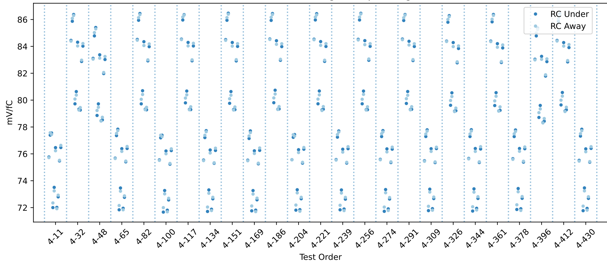
20USBHX2008046 RC gain chip averages
