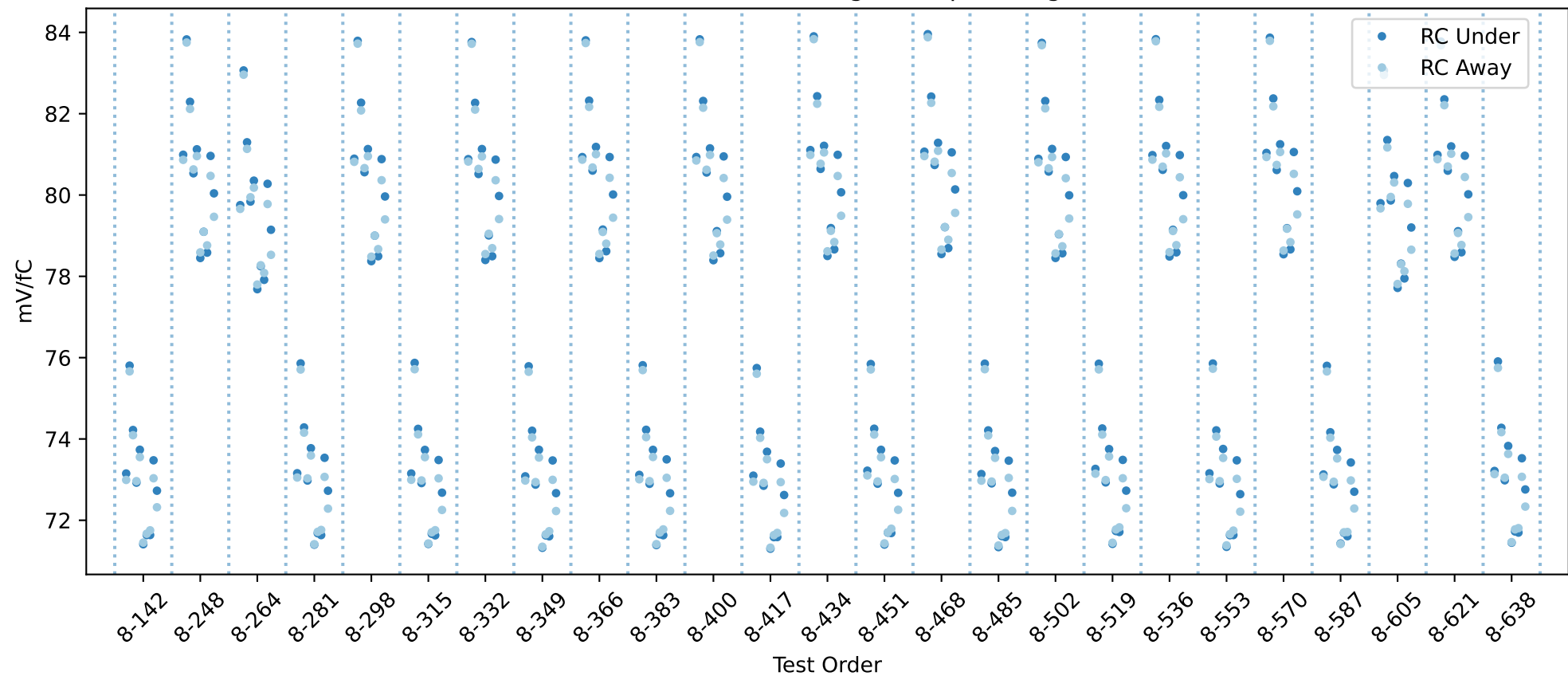
20USBHX2008048 RC gain chip averages
