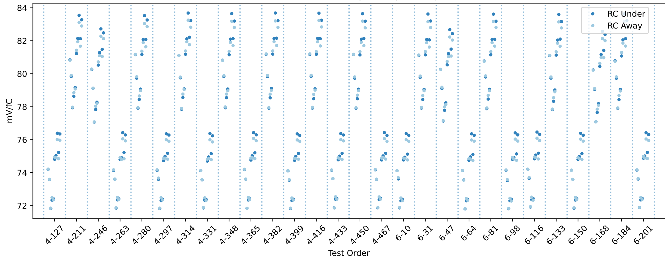
20USBHX2008066 RC gain chip averages
