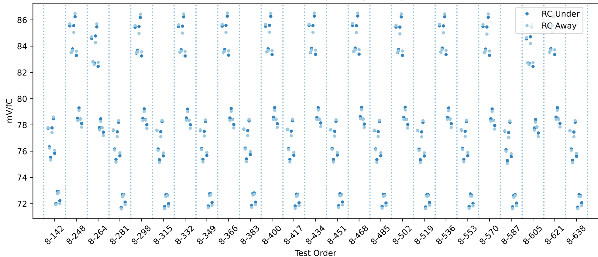
20USBHX2008017 RC gain chip averages
