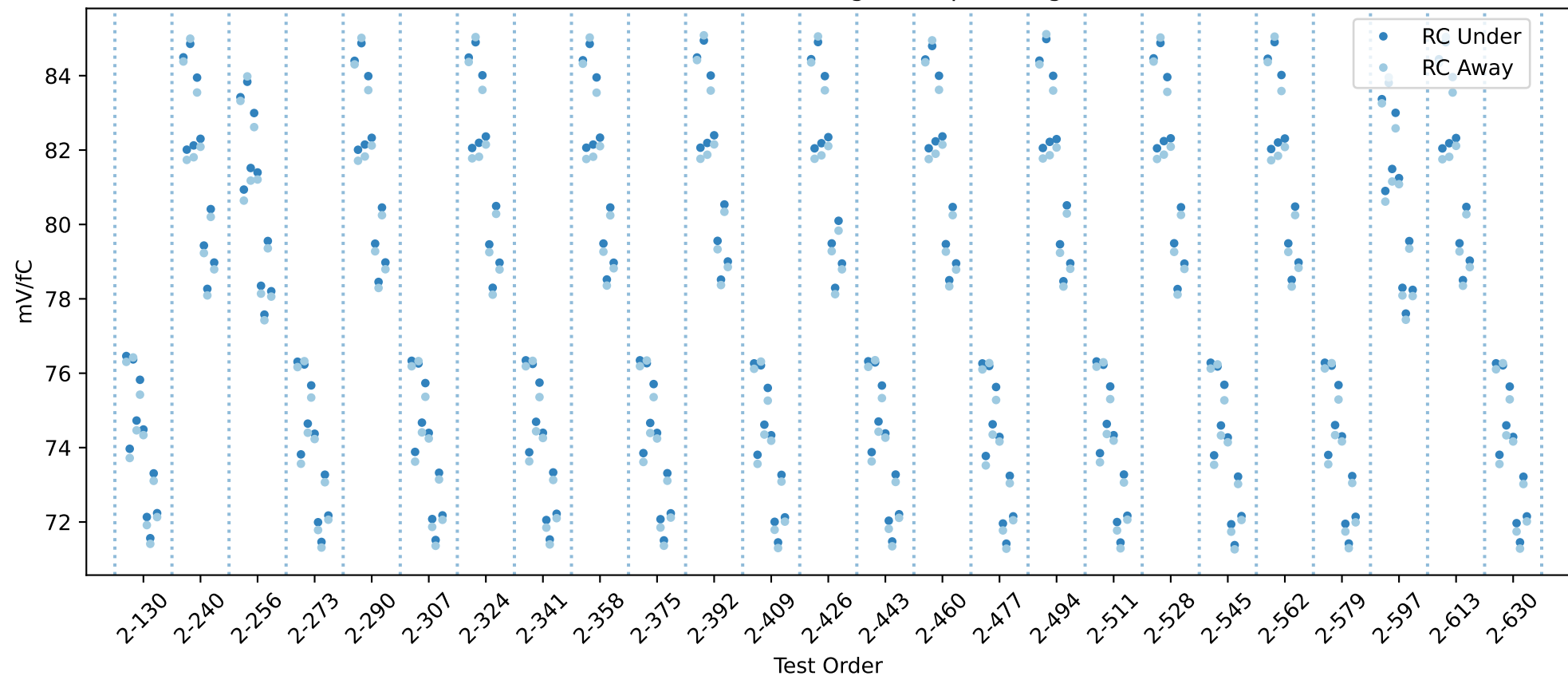
20USBHX2008101 RC gain chip averages
