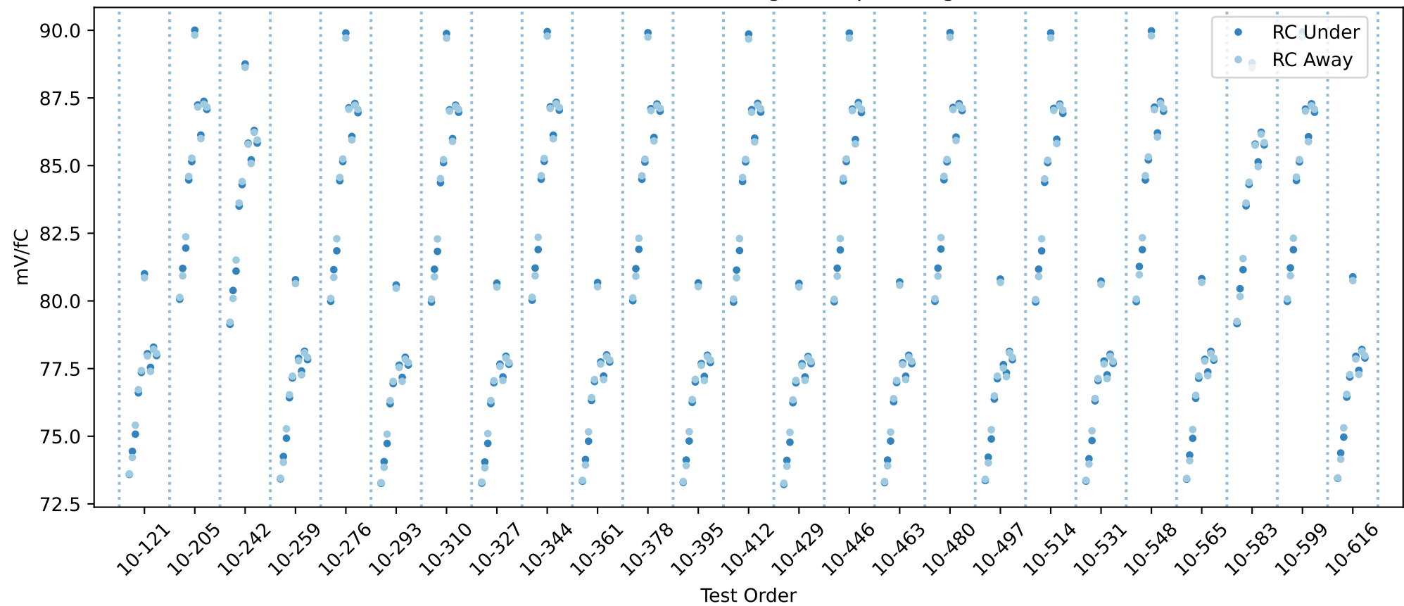
20USBHX2008116 RC gain chip averages
