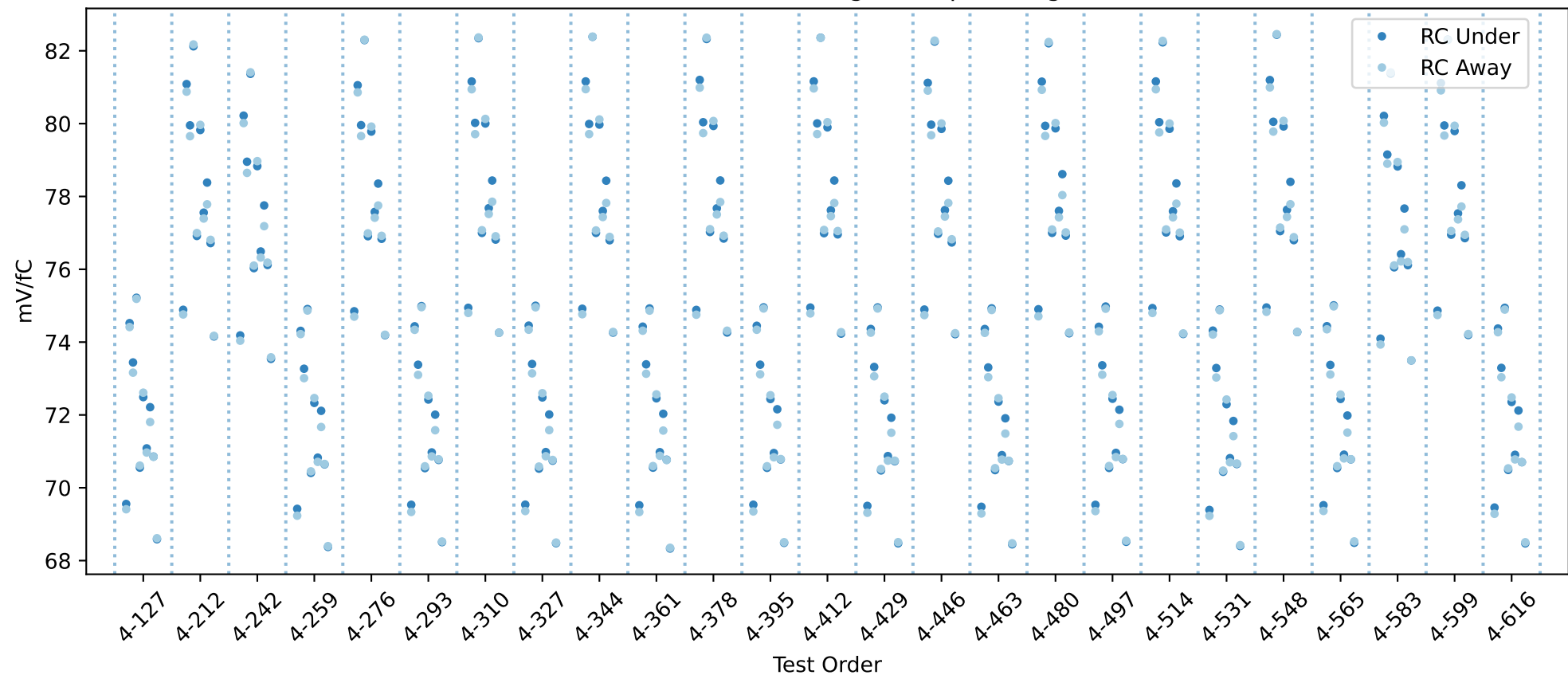
20USBHX2008113 RC gain chip averages
