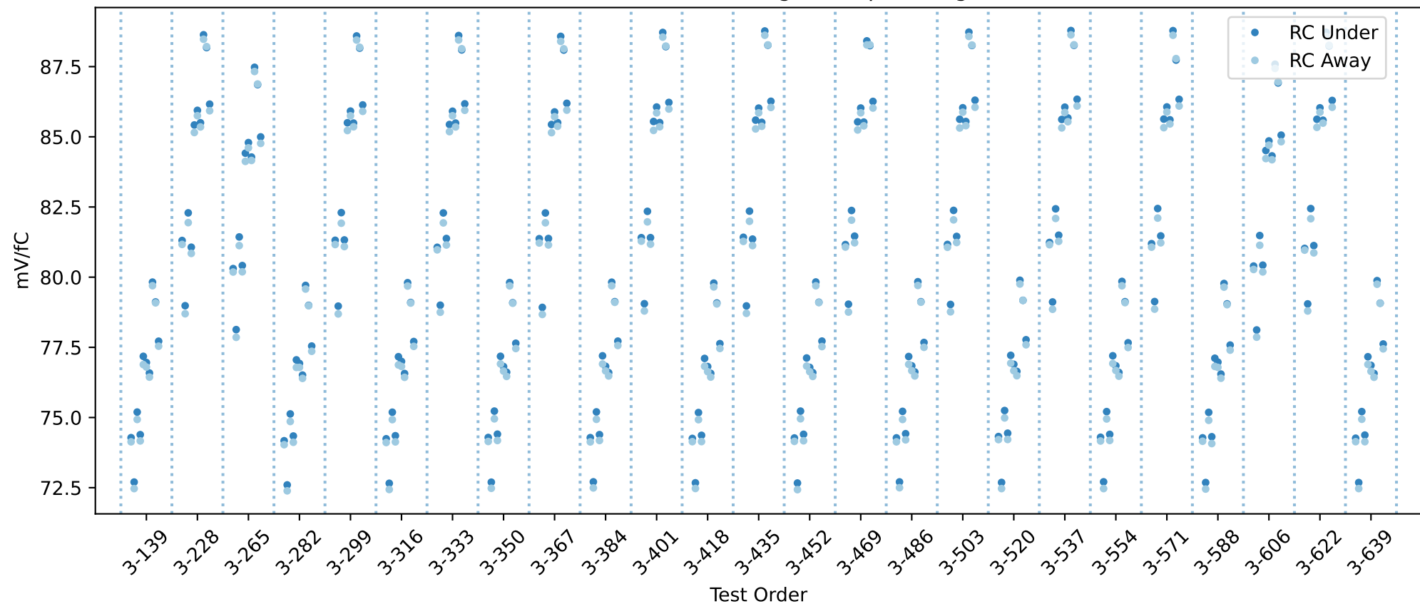
20USBHX2008124 RC gain chip averages
