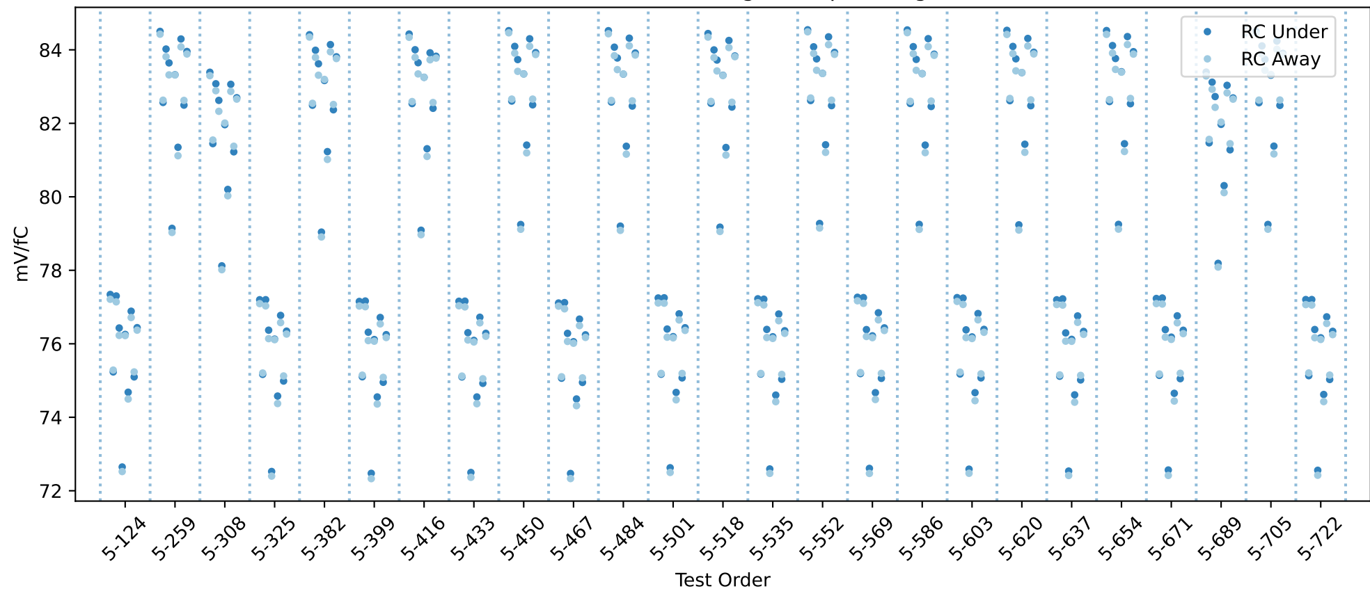
20USBHX2008087 RC gain chip averages
