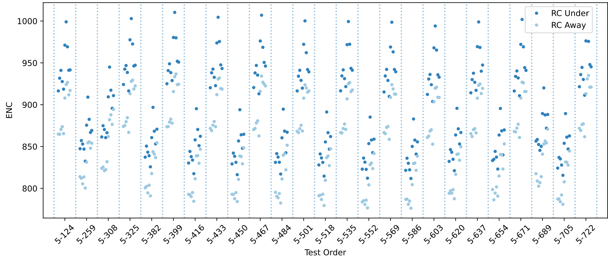
20USBHX2008088 RC innse chip averages
