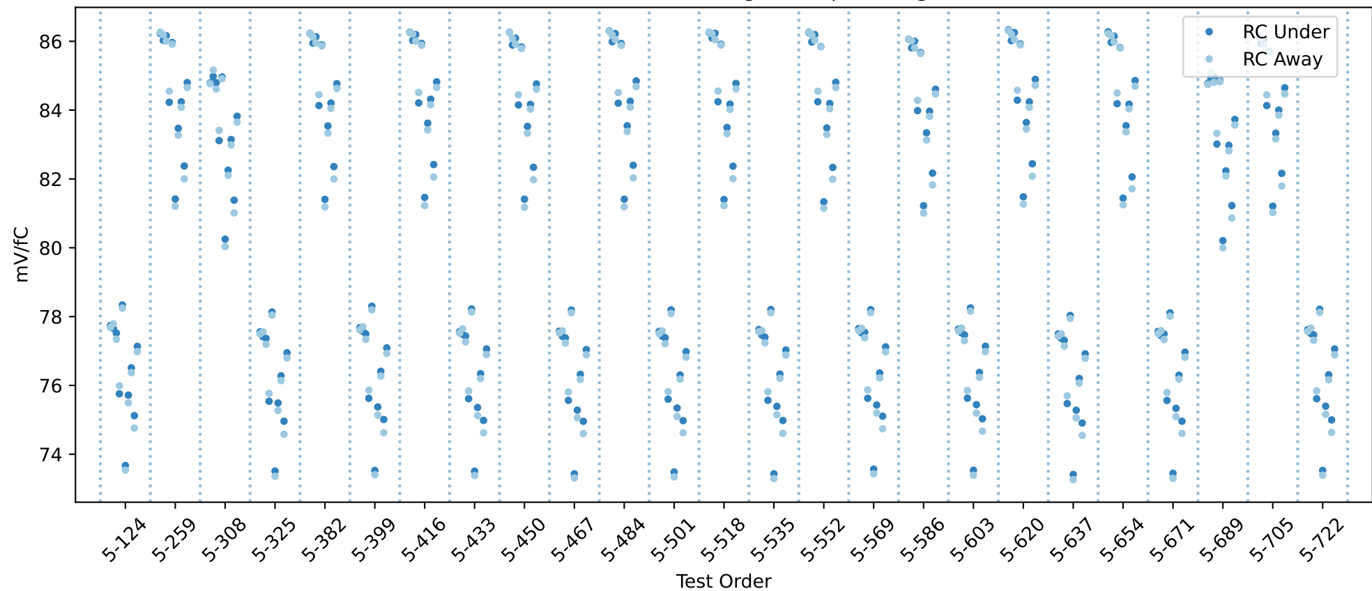
20USBHX2008089 RC gain chip averages
