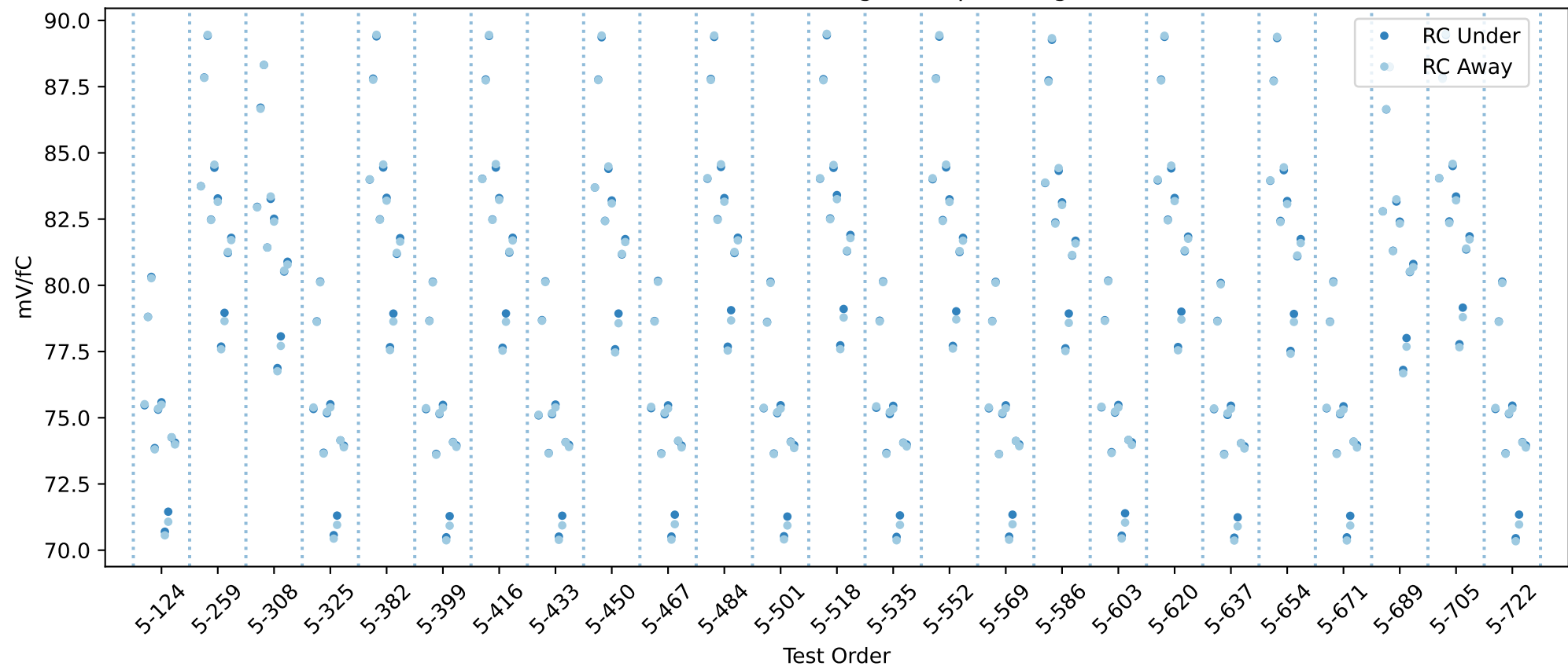
20USBHX2008090 RC gain chip averages
