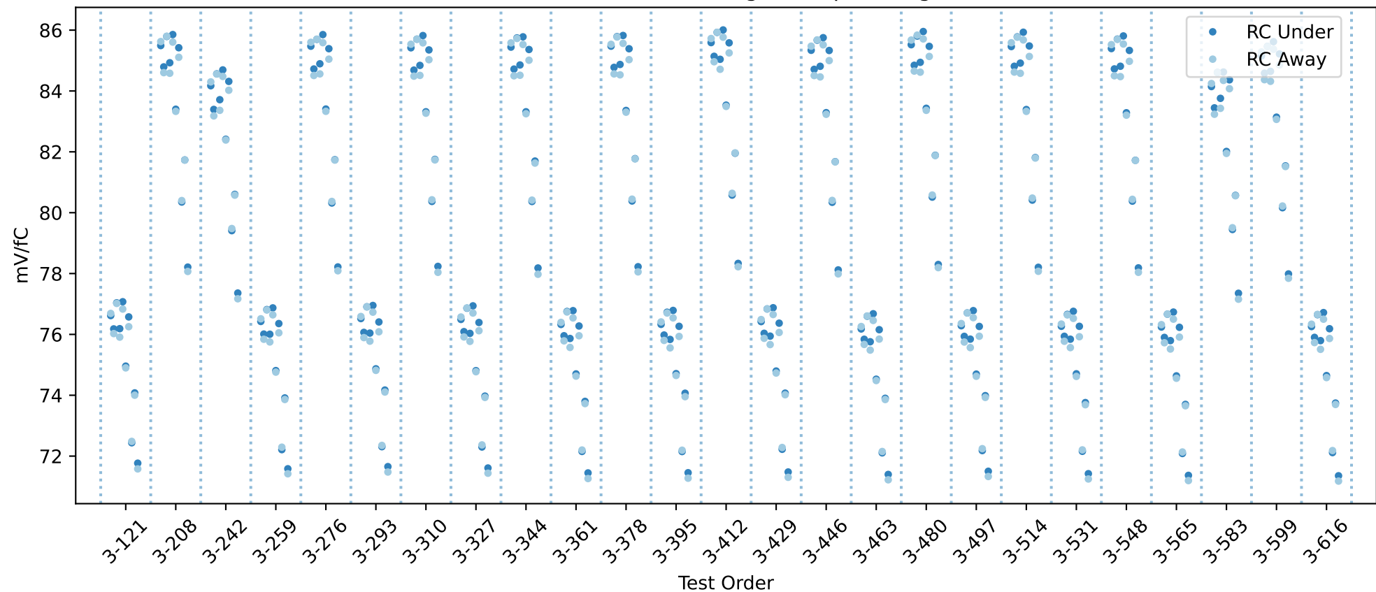
20USBHX2008119 RC gain chip averages
