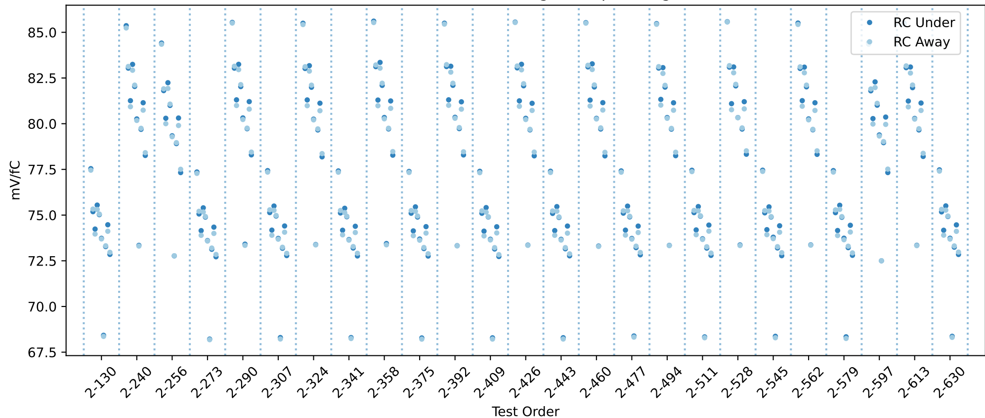
20USBHX2008070 RC gain chip averages
