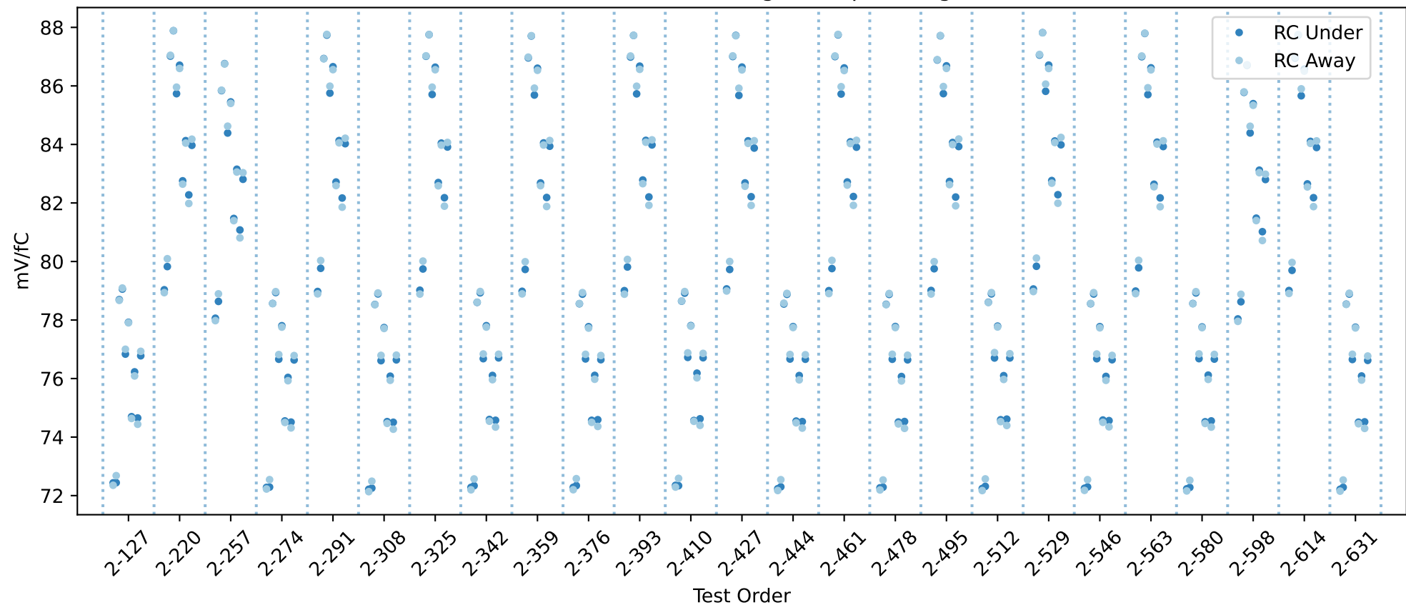
20USBHX2008093 RC gain chip averages
