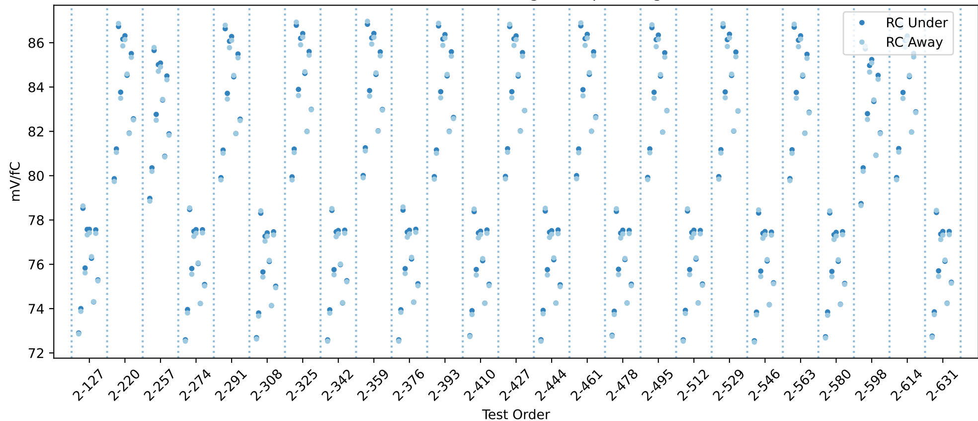
20USBHX2008095 RC gain chip averages
