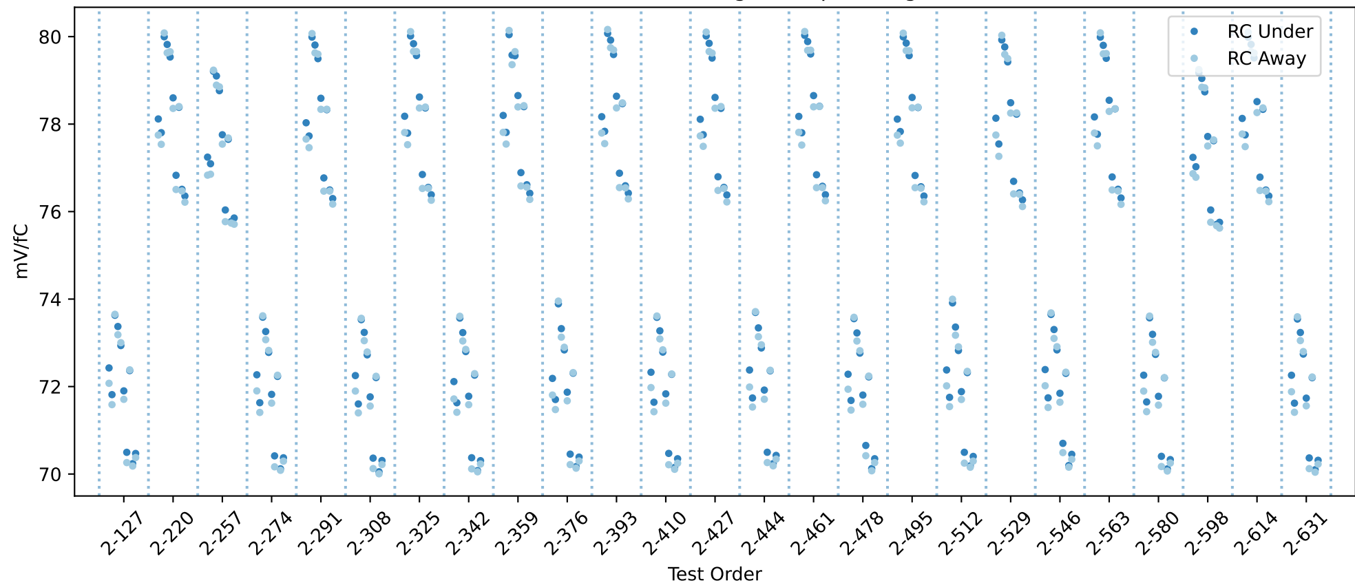
20USBHX2008049 RC gain chip averages
