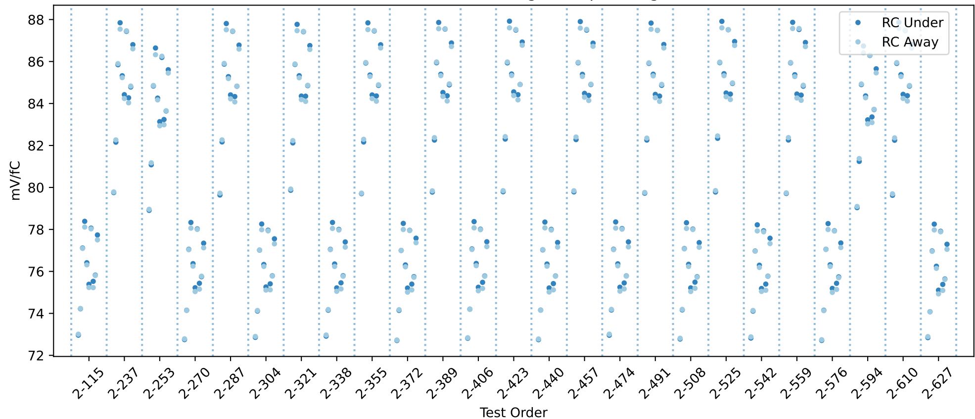
20USBHX2008141 RC gain chip averages
