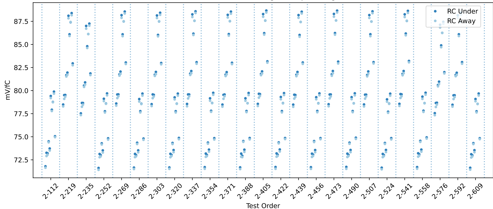
20USBHX2008128 RC gain chip averages
