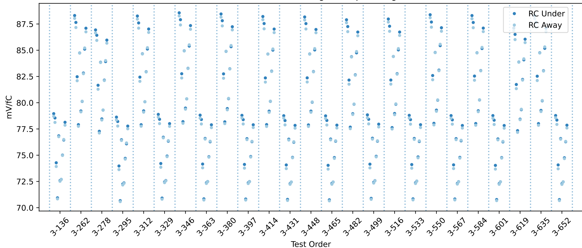
20USBHX2008149 RC gain chip averages
