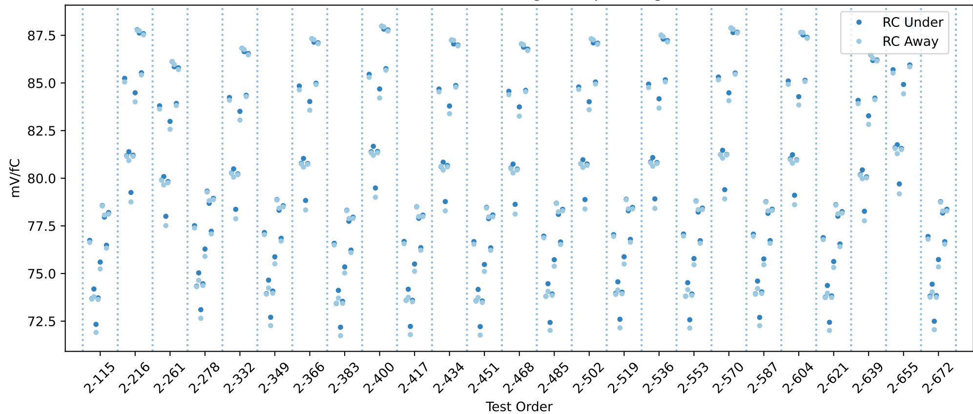
20USBHX2008099 RC gain chip averages
