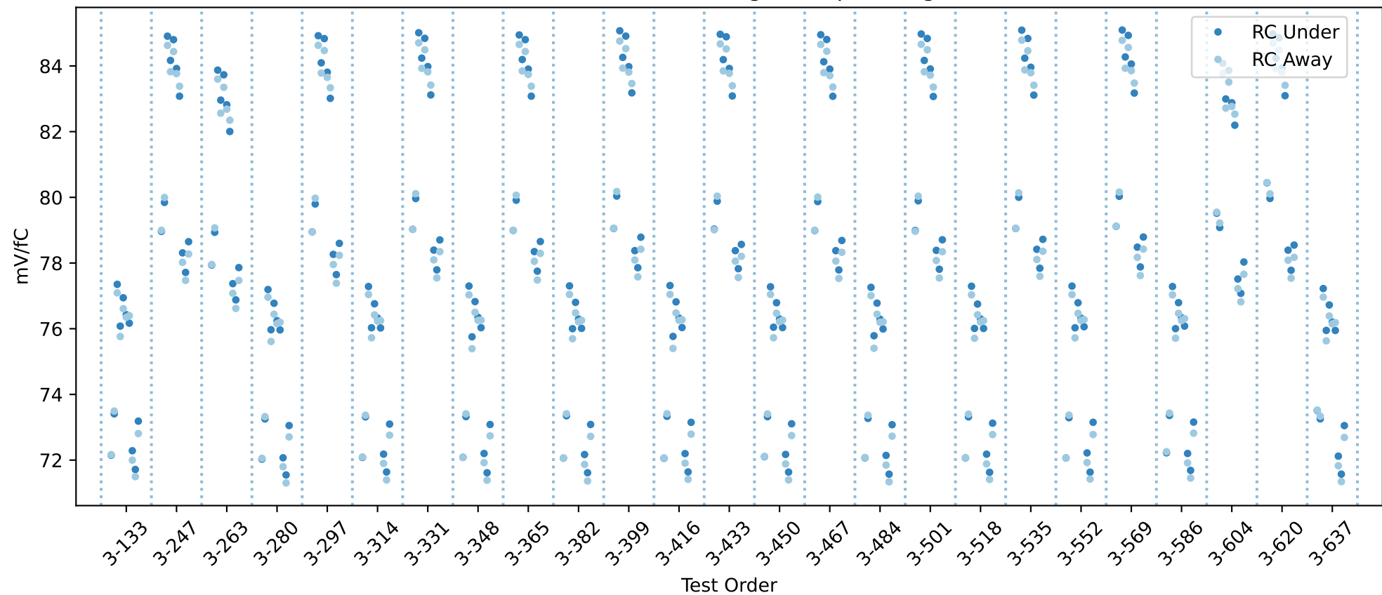
20USBHX2008084 RC gain chip averages
