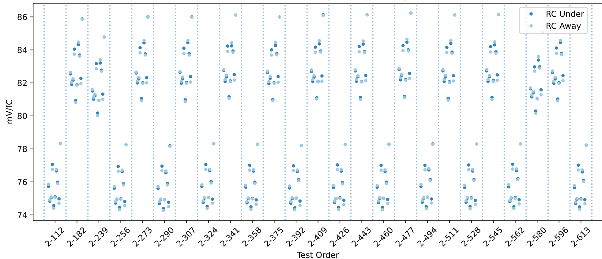
20USBHX2008078 RC gain chip averages
