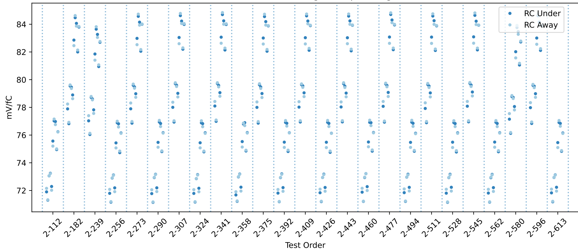
20USBHX2008079 RC gain chip averages
