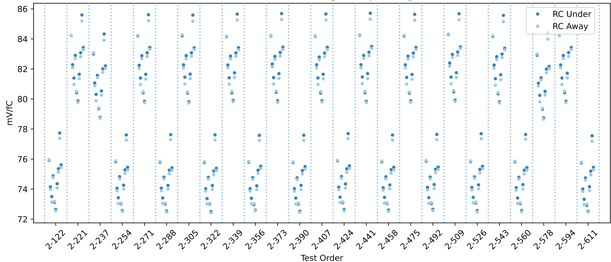
20USBHX2008432 RC gain chip averages
