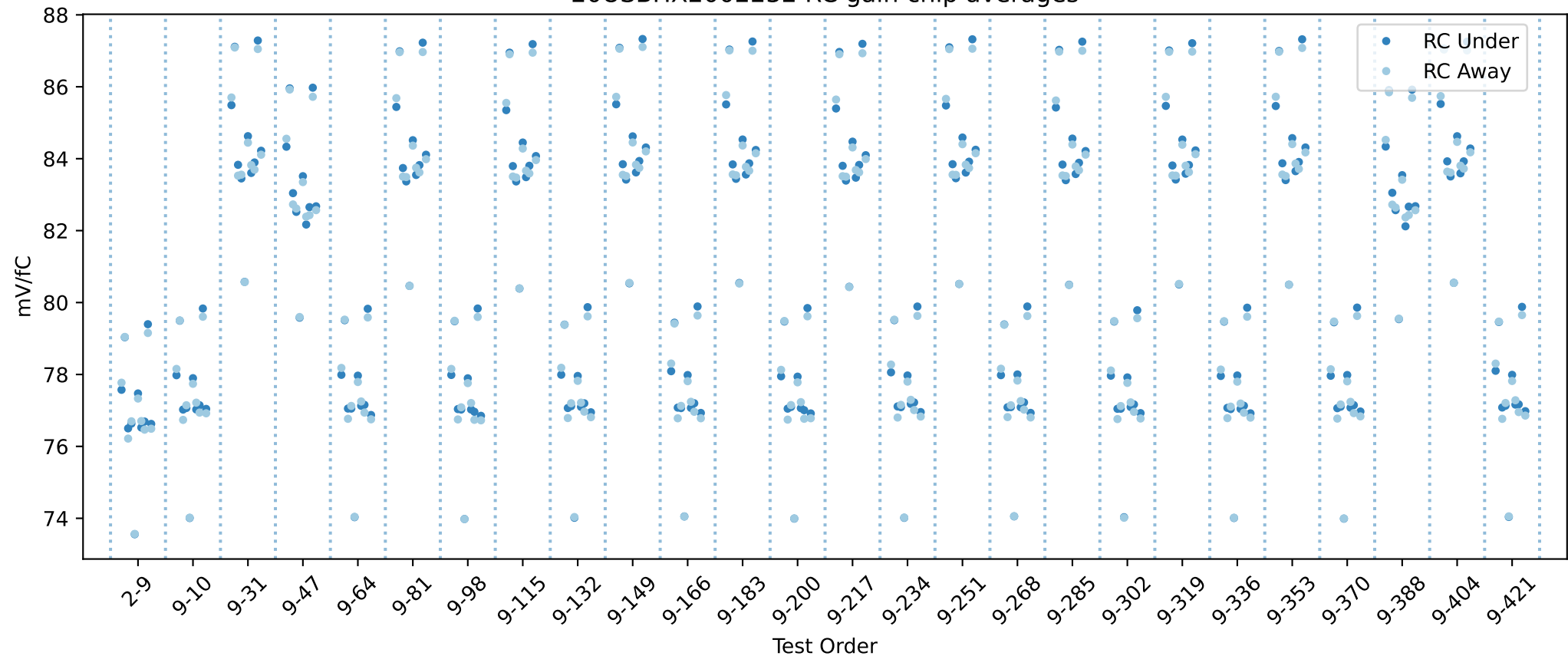
20USBHX2002232 RC gain chip averages
