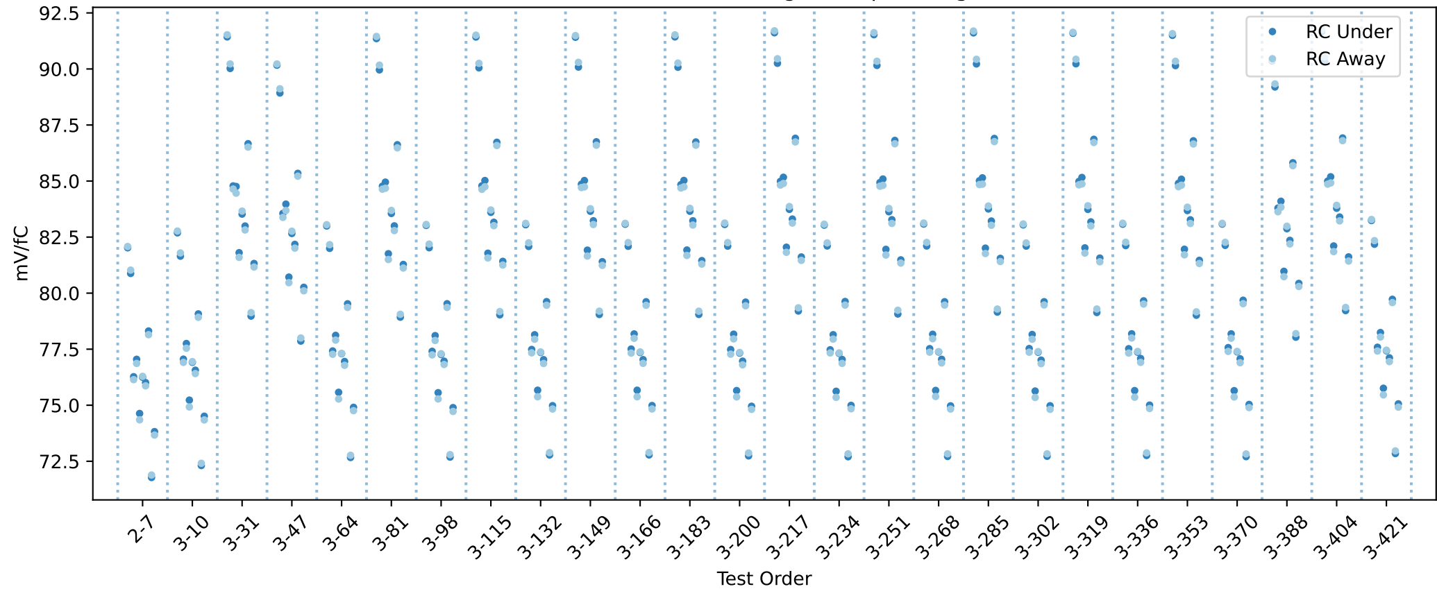
20USBHX2002235 RC gain chip averages
