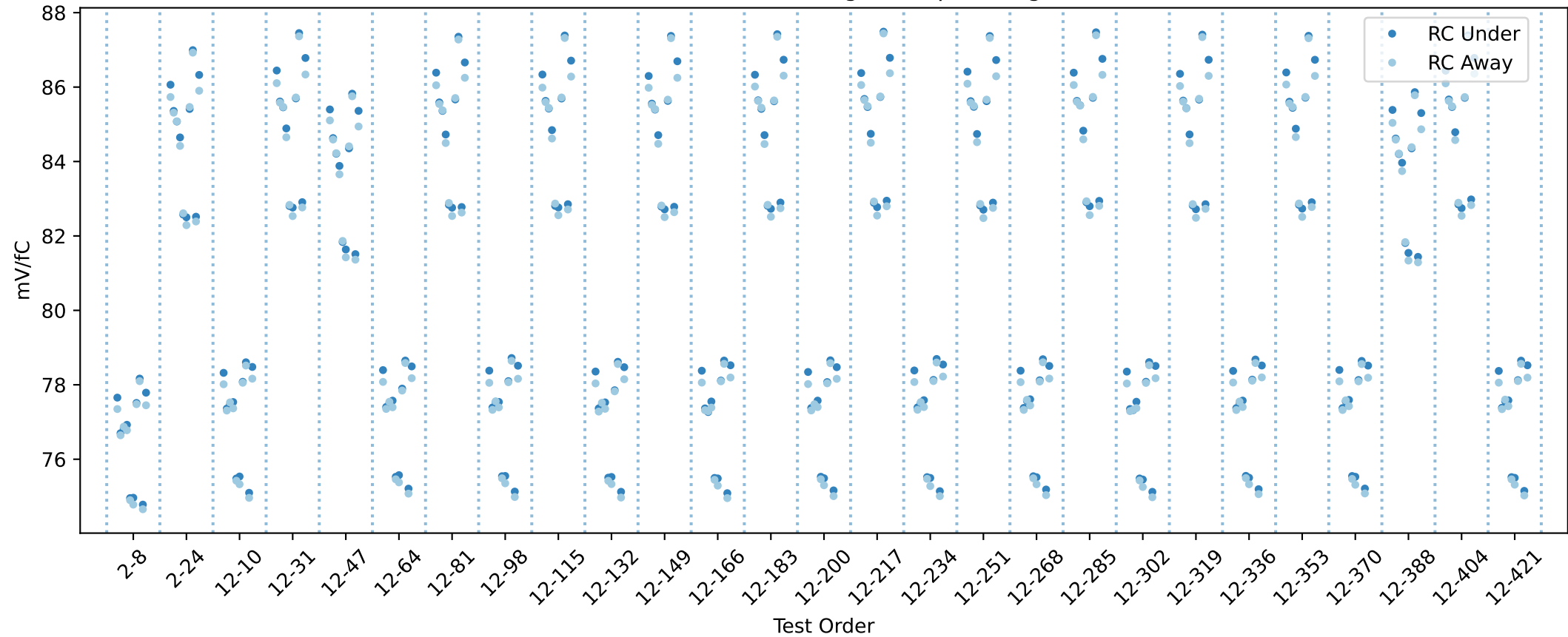
20USBHX2002239 RC gain chip averages
