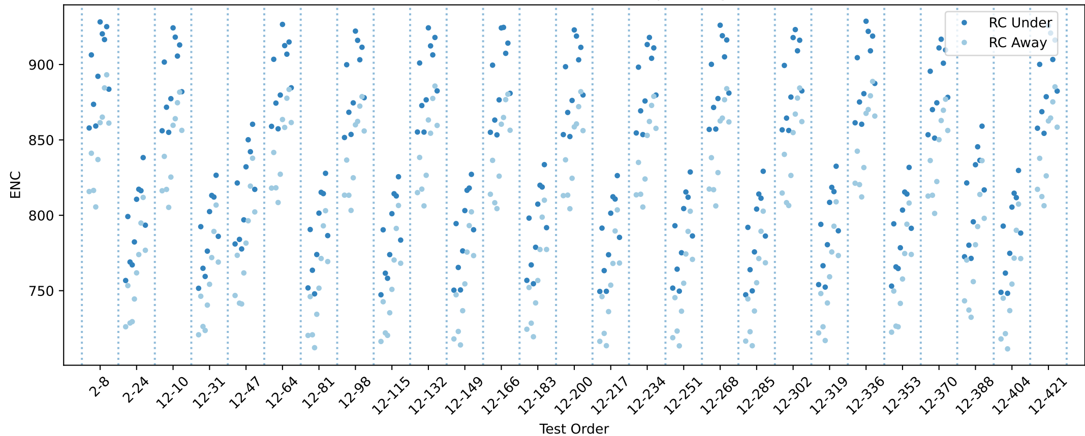
20USBHX2002239 RC innse chip averages
