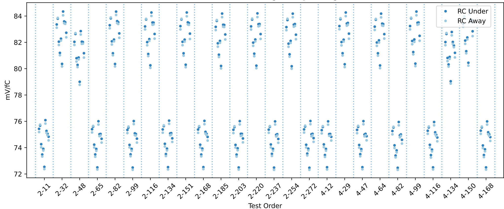
20USBHX2002508 RC gain chip averages
