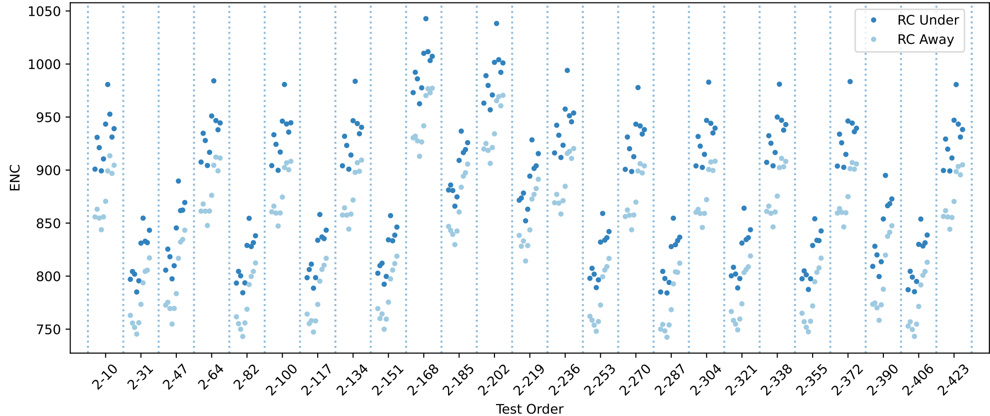
20USBHX2002504 RC innse chip averages
