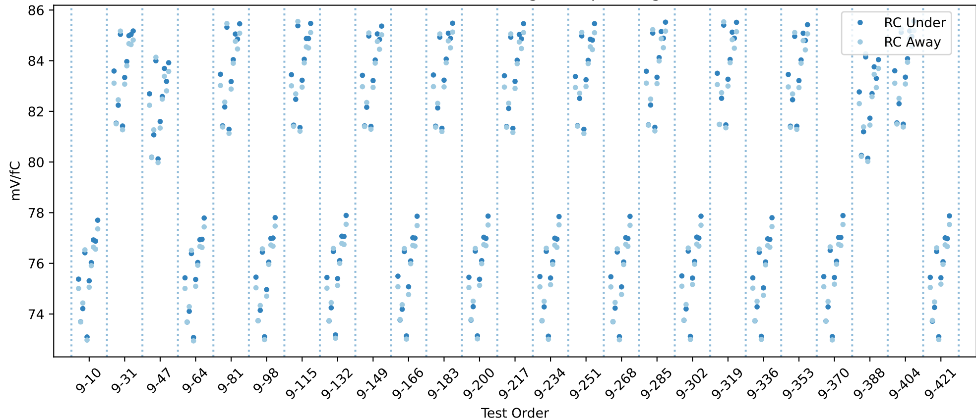
20USBHX2002505 RC gain chip averages
