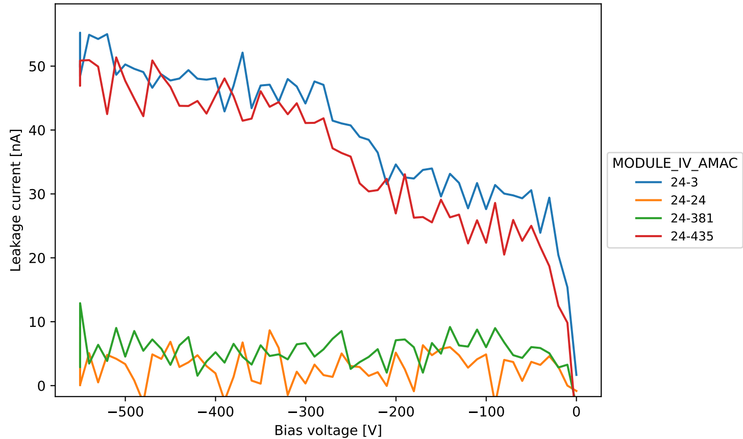
20USBML1235684 standard IV
